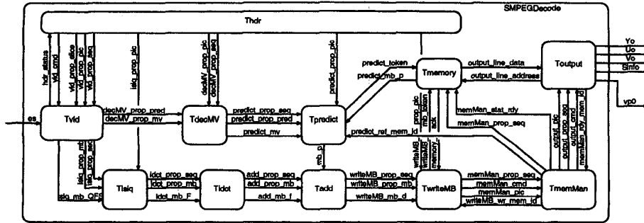
Figure 1: MPEG decoder
