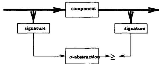
Figure 3: \sigma -abstraction must be conservative.
